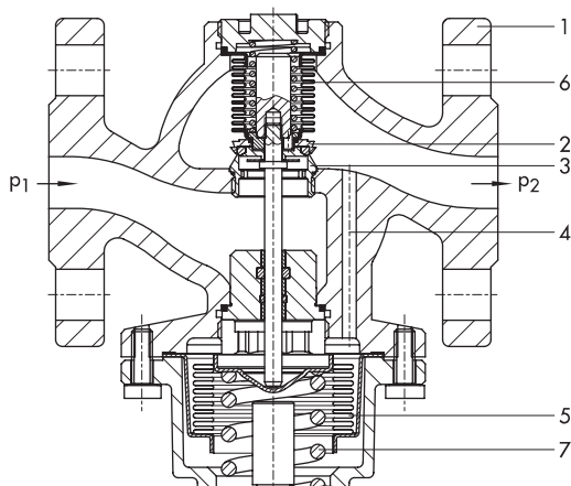
Types 44-0 B, 44-1 B Pressure Reducing Valves Flanged body (spheroidal graphite iron)
