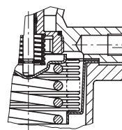
Special version of Type 44-1 B or Type 44-6 B Regulators prepared for connection of a pressure gauge or external control line
