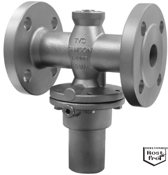
Fig. 1 · Type 44-1 B Pressure Reducing Valve, flanged body made of stainless steel
