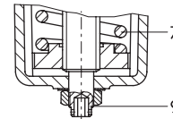
Version of stainless steel or spheroidal graphite iron (DN 40 and 50 only) and 8 to 20 bar set point range Set point adjusted at a hexagon socket screw
